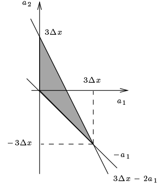
Figure 4: Region satisfying the x constraints
