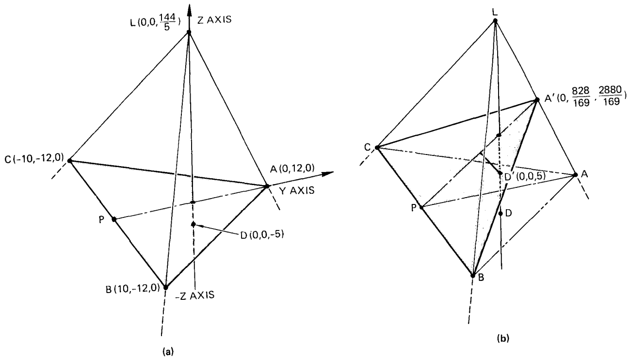
Fig. 6. An Example of a P4P Problem with Two Solutions.
