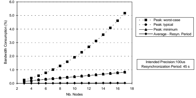
Figure 7. Bandwidth consumption (T=45s)
